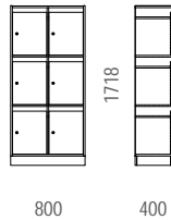
W250-32 Locker with letter boxes
