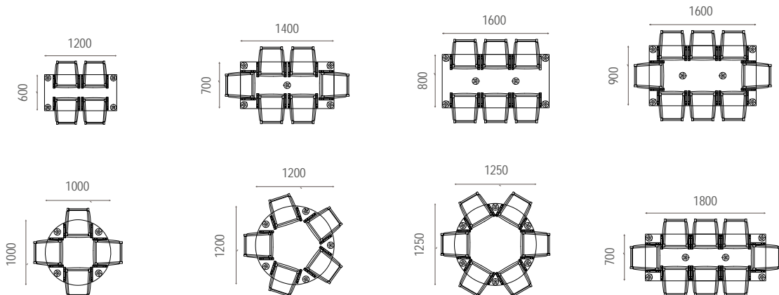
The suspension of the O100 adult's Onni chair underneath tables with flange legs.
